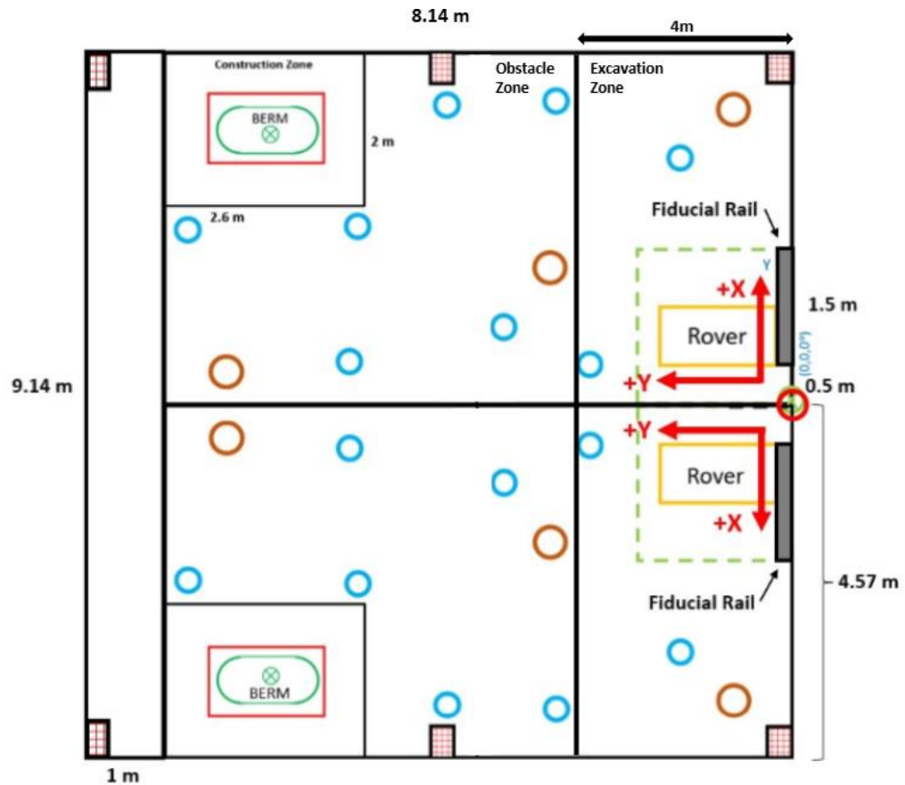
Figure 1: UCF Arena Layout (new layout for 2026 may still be adjusted further forward, away from ingress door based on testing)
